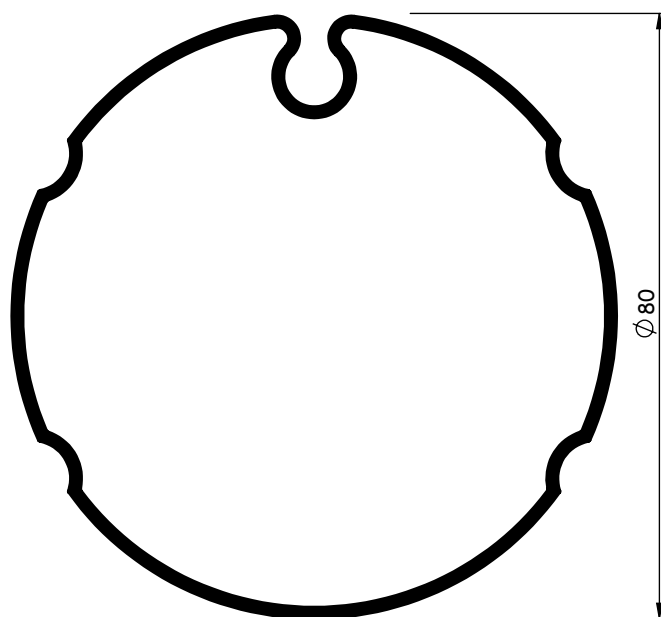
AL905 0,998 - 1,219 kg/m
