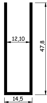
AL343 1,203 - 1,227 kg/m
