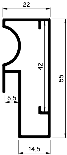
AL1528P 0,520-0,600 kg/m
