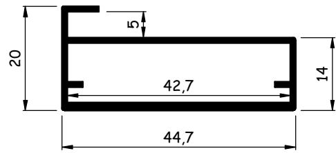
AL1502 0,459 kg/m
