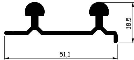
AL1510 0,553 kg/m
