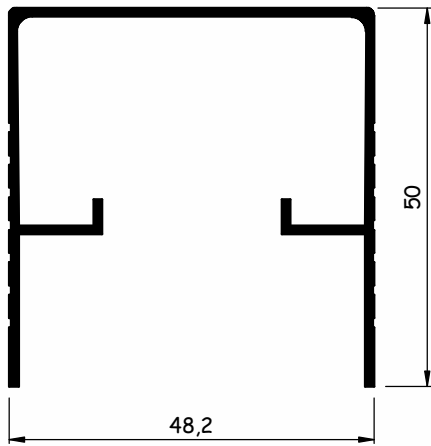
AL041C-P (BX-183) 0,554 kg/m
