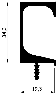
AL1530 (BK-501) 0,540 kg/m
