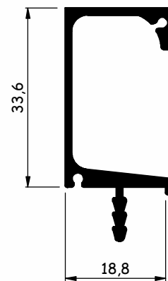
AL1533 0,398 kg/m
